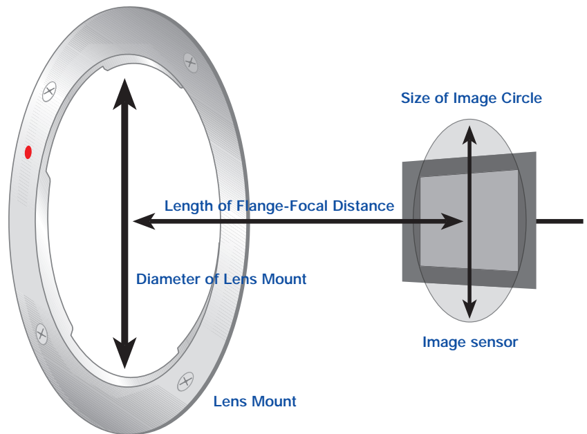
The Four Thirds System standardizes the diameter of the lens mount, the size of the image circle, the flange-focal distance, and more.
